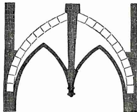
Figure 8. English vault ( \alpha:6 ) with hanging keystone resisting tension to retransmit the loads to the real vault.
