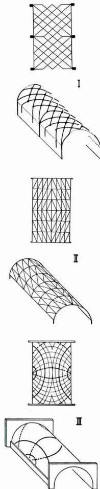
Figure 47. Schemes of barrel vaults realized with different techniques and materials: I, reticulated Gothic vault in stone and brick material acting well in resistance only to compression; II, reticulated metallic vault, in material which is best for resistance in tension; III, thin shell in ordinary reinforced concrete with dotted lines indicating the tension isostatics and continuous lines the compression isostatics. In this last the edge beams and the frontal diaphragms are necessary members.
