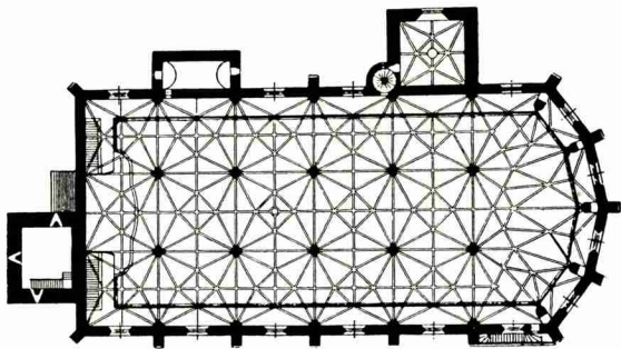
Figure 30. Plan of the church of Schneberg in Saxonia, where the three naves are founded in a unified atmosphere and the vaults collaborate in a unified static behavior.
