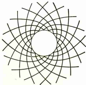
Figure 51. Orthogonal logarithmic spirals as lines of stress (from Nadai).
