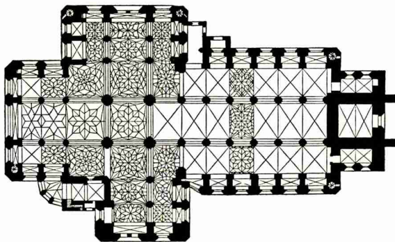
Figure 28. Plan section of the Church of Maria at Danzig with the projection of the ribworks of the most complicated vaults dating from the beginning of the 15th century.
