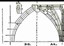
Figure 7. Geometrical generation and appearance of the star vault ( \alpha:1 ); furnished, that is to say, at every support with two "tiercerons" in addition to the ogive. The prolongations of the "tiercerons" which form the sides of the octagon take the name of "false-liernes." While "ridge-liernes" are the arches following the centers.
