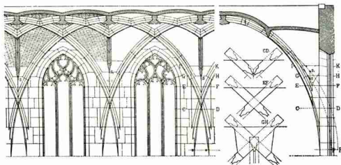
Figure 39. Longitudinal and transverse sections of the reticulated vault in the church of the Madonna at Leinsingen. Note the different elevations of the supports of the various diagonal and orthogonal ribwork.
