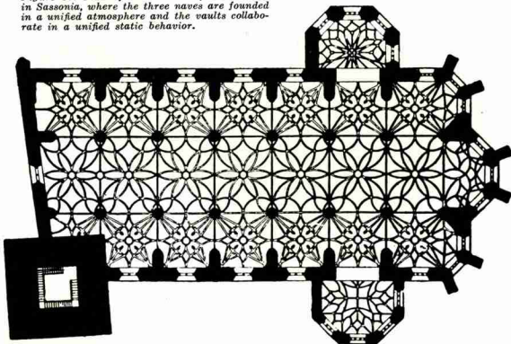
Figure 31. The Church of St. Anna at Annaburg built between 1499 and 1520 by Bartol von Durbach and Konrad von Buitgen. The vision of the whole of the tracery of the ribwork is necessary for the comprehension of the architectonic composition and of the statics of the boldest structure.
