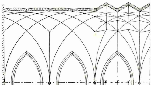
Figure 40. Difference between a reticulated vault "netzgewölbe" and cellular vault "zellengewölbe" consisting only in the minor or major concavity of diaphragms placed to stiffen the small nets of the principal reticulation of the ribwork.
