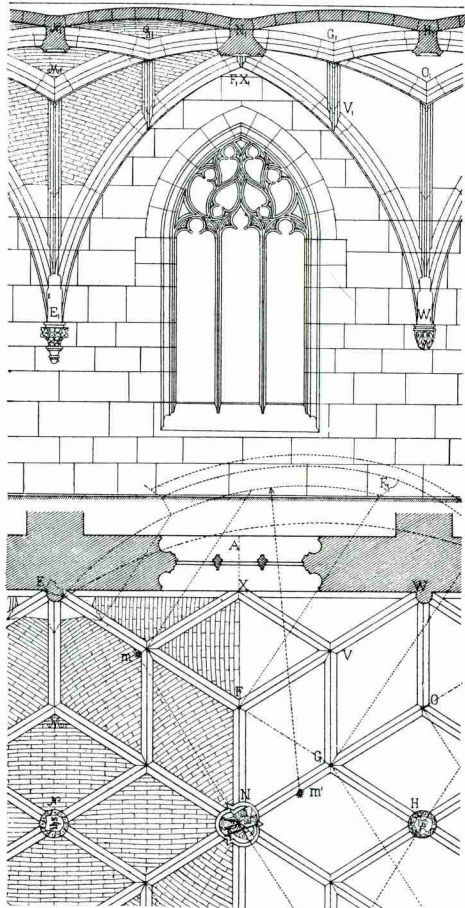
Figure 11. Reticulated vault, called by the Germans "netzgewölbe" in the Oratorio of Maulbronn. The sections of the secondary vaults and their dispositions are very instructive concerning the static regimen of the structural complex. The claw projections on the windows resolve, besides an architectonic problem relating to the illumination, a static exigency of eliminating the zones in which the ribs would have worked in tension.
