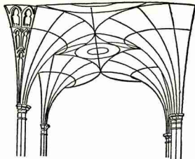
Figure 12. Generative scheme (a:∞) of the vaults of Kings College.
