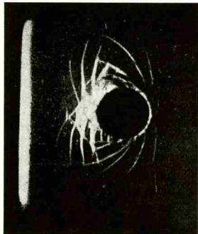
Figure 50. Figure of Krüger, lines of stress in a sheet of iron compressed from a small cylinder.
