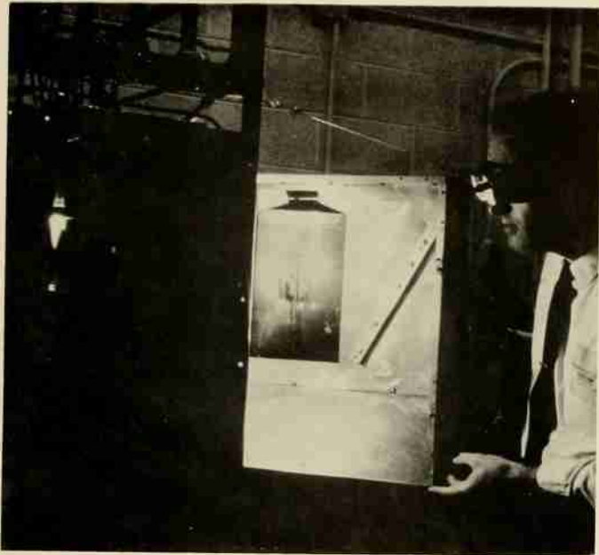
A ceramic experiment carried out in the heat of RF plasma crystal growing facility is seen by Dr. Palmour.
