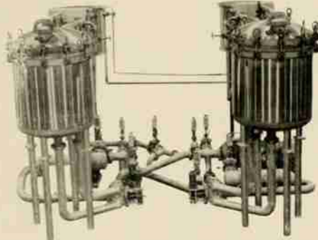
Two 'Single Kier' 500 pound Dyeing Machines with 'criss-cross' Tandem System
