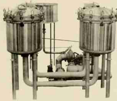
'Twin-Kier' 1500 lb. Package Dyeing Machine
