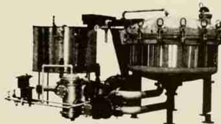
Single Kier Pressure Dyeing Machine
