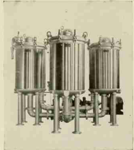
Multiple-Kier Beam and Package Dyeing Machine
