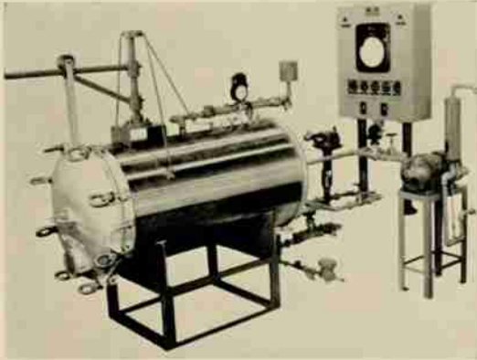
Woolen and Worsted Yarns New "Hy-Vacuum" Pressure Autoclave for Nylon "Helanca"
