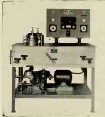
Laboratory Dyeing Machine
